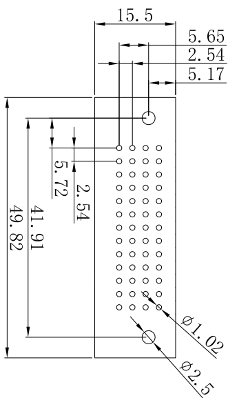
P.C. Body Hole Layout
